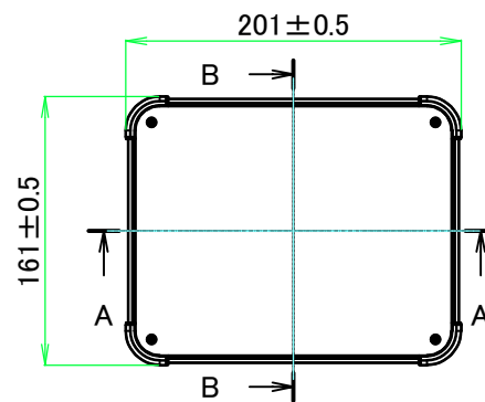
A view
