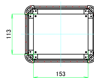
C-C (1:5)
